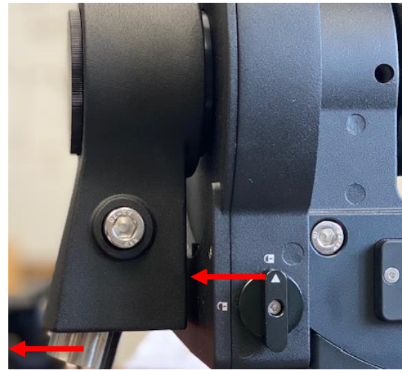
Figure 20. Tilt the counterweight shaft for low altitude
