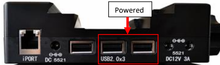
Figure 7. Ports on CEM70 dovetail saddle
