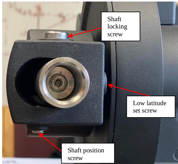
Figure 19. Screws for CW shaft tilting
