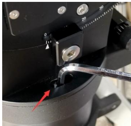
Figure 14. Locking the mount
