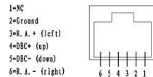
Figure 3. ST-4 port wiring
