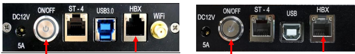
Figure 23. CEM70G (left) and CEM70/EC (right) mount base panel
