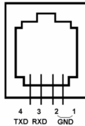
Figure 10. Serial port pin-out on an 8407+ hand controller
