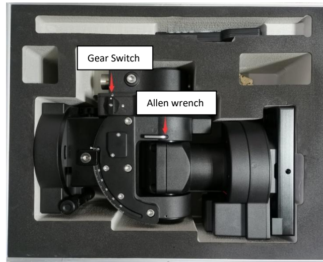
Figure 12. Remove the mount
