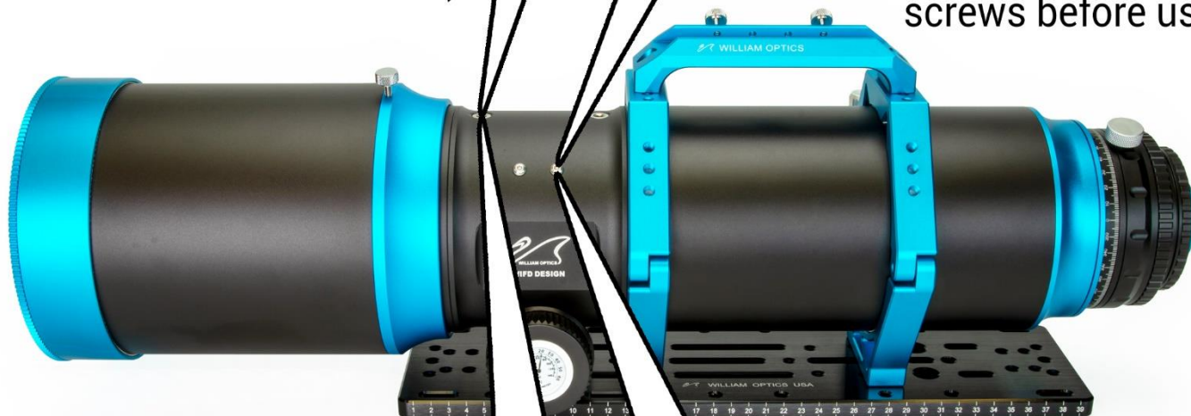
Tension Screws (for increase focuser tension)
