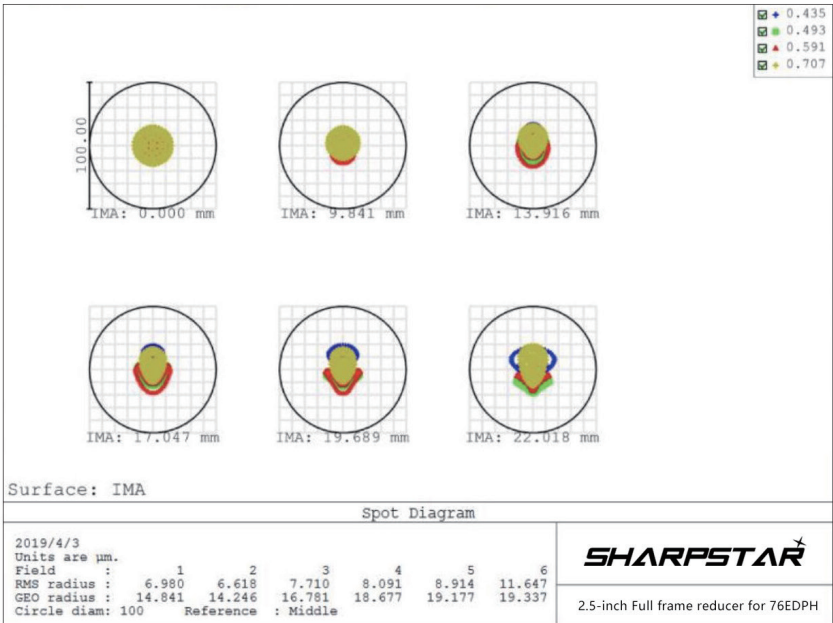
Spot diagram
