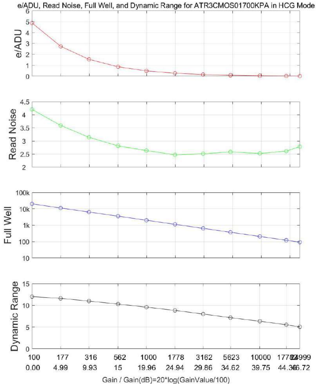
Figure 2 e/ADU, Read Noise, Full Well and Dynamic Range for ATR3CMOS01700KPA
