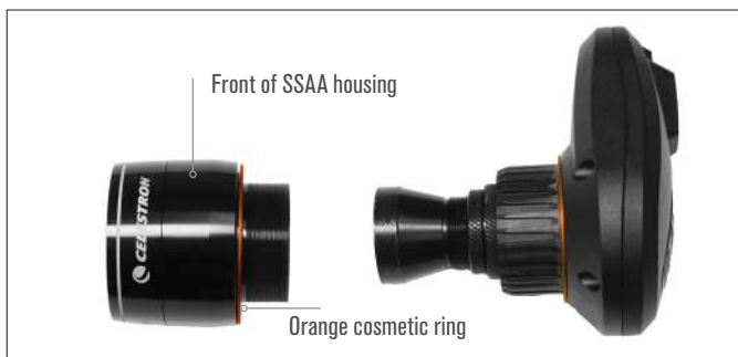
Fig. 6: To switch brackets, completely unthread and remove the entire front of the SSAA housing, including the orange ring.
