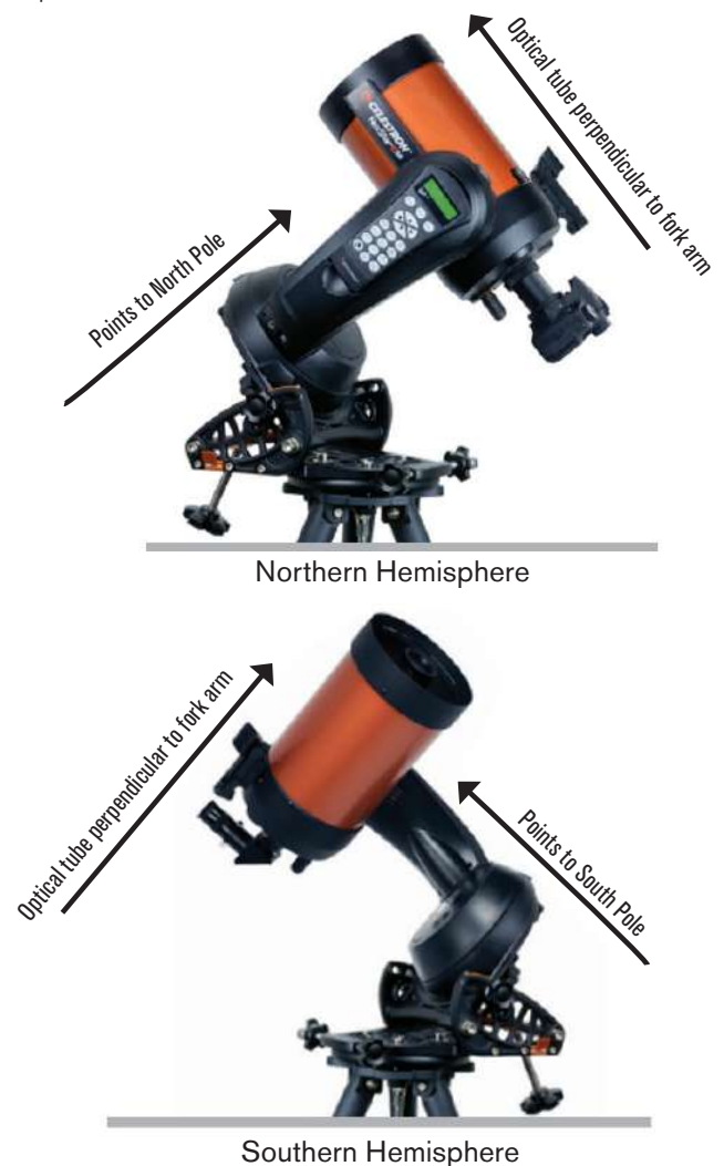
Fig. 12: When using an altazimuth (AZ) fork mount on an equatorial wedge, begin with the mount in the position shown. The fork arm should point due North (or due South in the Southern Hemisphere), and the optical tube should be perpendicular to the fork arm.
