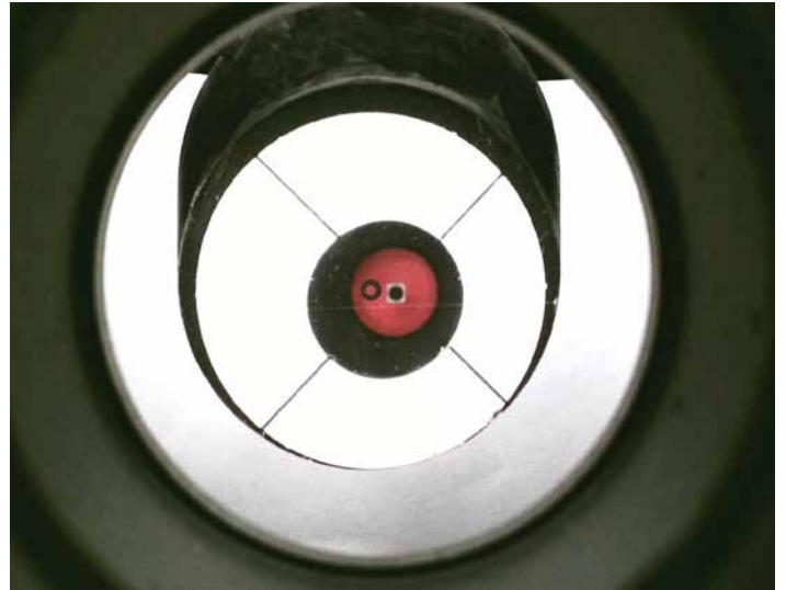
Figure 2 Rotate the secondary mirror (360° rotational axis) Face the secondary mirror toward us; approximate positioning is sufficient.
