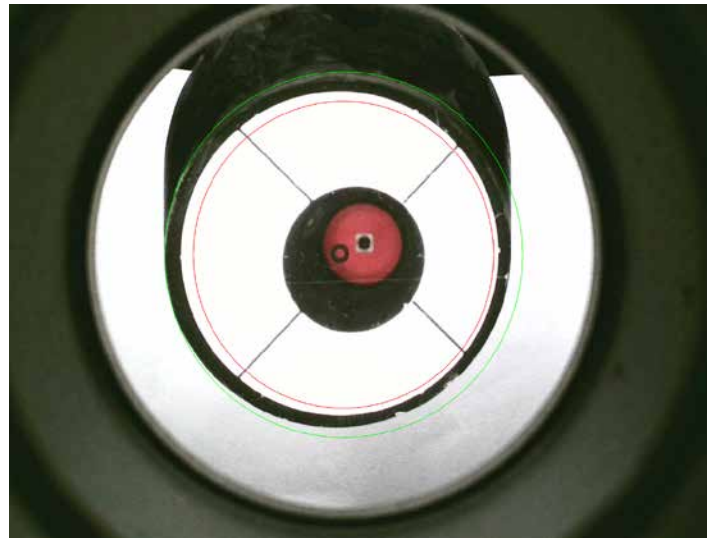
Figure 4 It can be seen from Figure 3 that the red circle has a large vertical elevation deviation from the primary mirror. In this case, use screw A to adjust the elevation angle of the secondary mirror.
