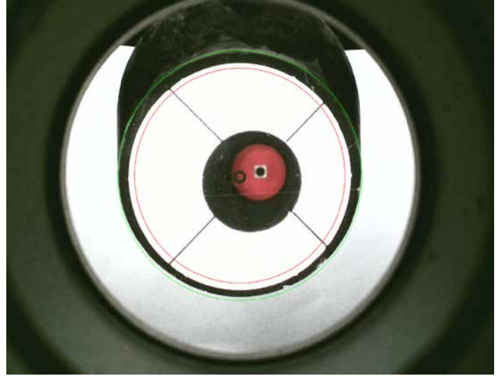
Figure 9 Adjust screw A. At this point, the secondary mirror is fully adjusted.
