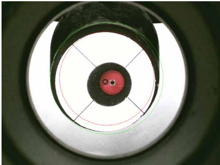
Figure 3 Turn on the red and green circles in the software. Adjust the red circle to approximately the same size as the primary mirror, and adjust the green circle to approximately the same size as the edge of the secondary mirror.
